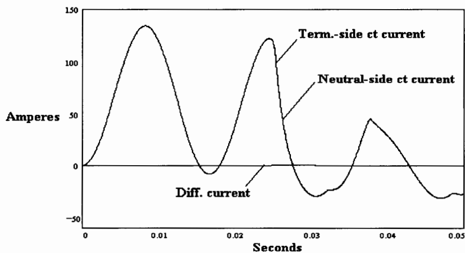
Figure 16—Secondary current in neutral and terminal side cts with differential current for corrected burden
