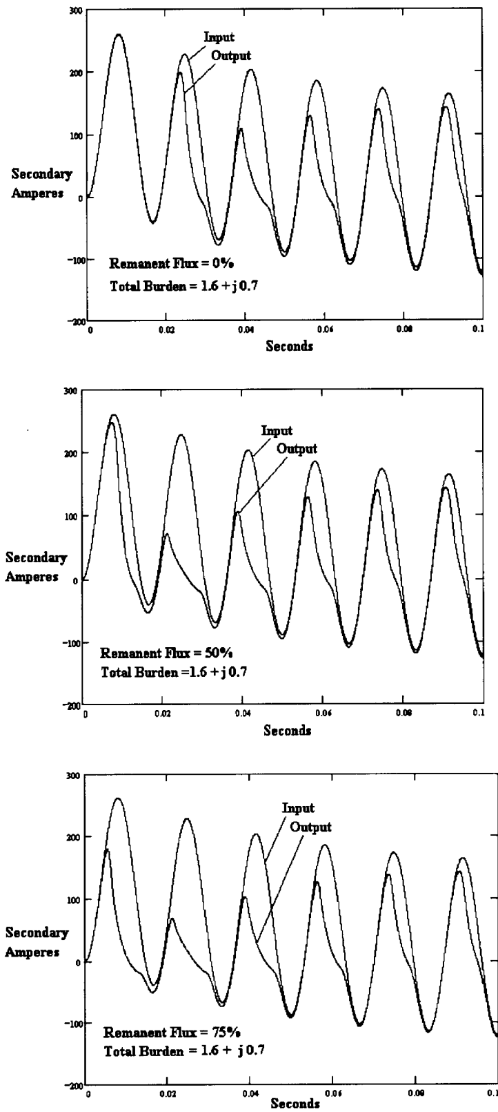
Figure 8—Secondary waveforms with increasing remanent flux
