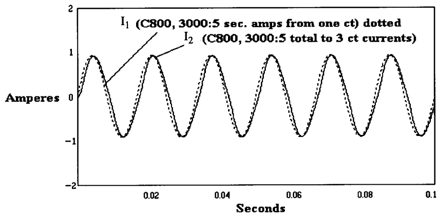
Figure 26—Secondary current for a 500 A minimum internal fault, bus differential relay with 400 V, 2210 Ω setting
