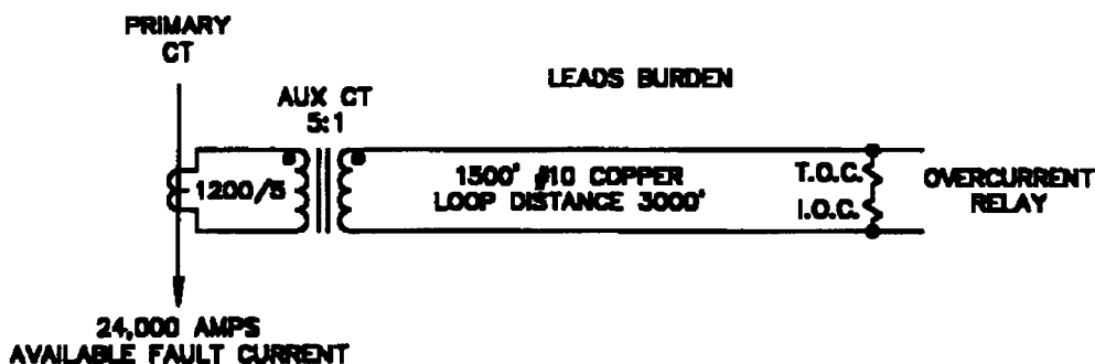
Figure 9—Burden calculation
