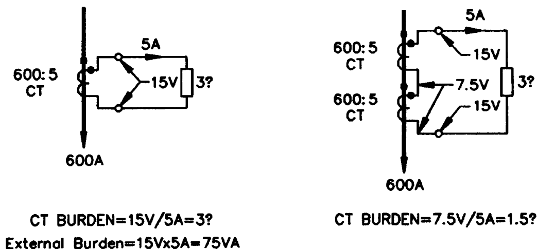
Figure 10—CT connected in series
