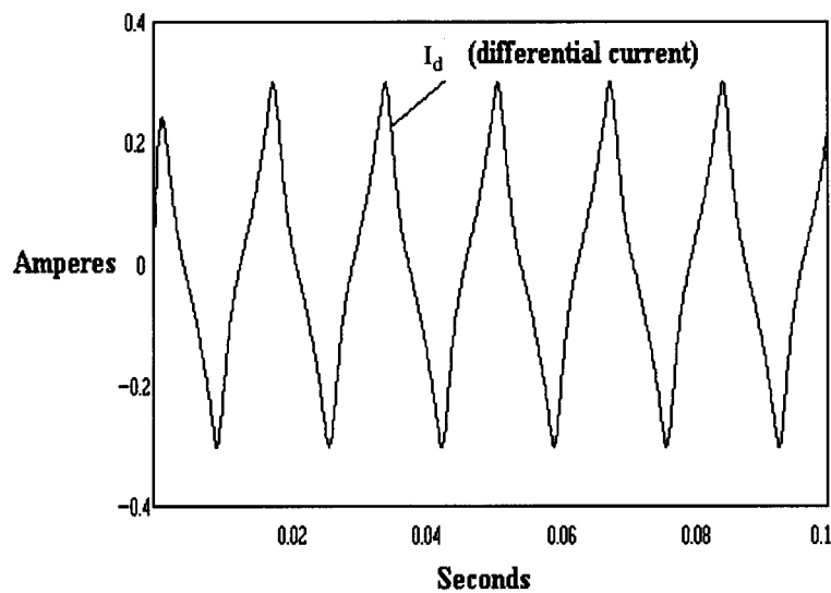
Figure 27—Operating current in a high-impedance bus differential relay (trip level 0.255 A peak) for a 500 A four-breaker bus
