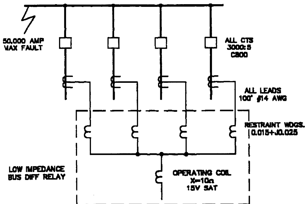
Figure 28—Low-impedance bus differential application
