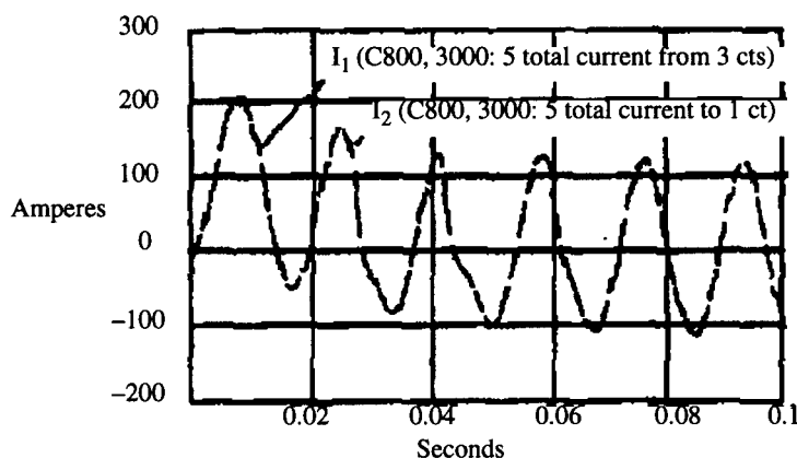
Figure 24—Secondary current for a 50 000 A external fault, bus differential relay with a 400 V 2210 \Omega setting
