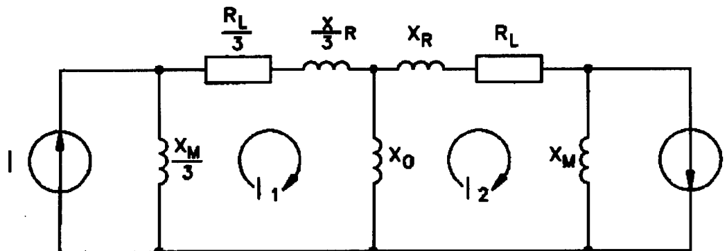
Figure 23—Equivalent circuit of 3 cts supplying current to 1 ct
