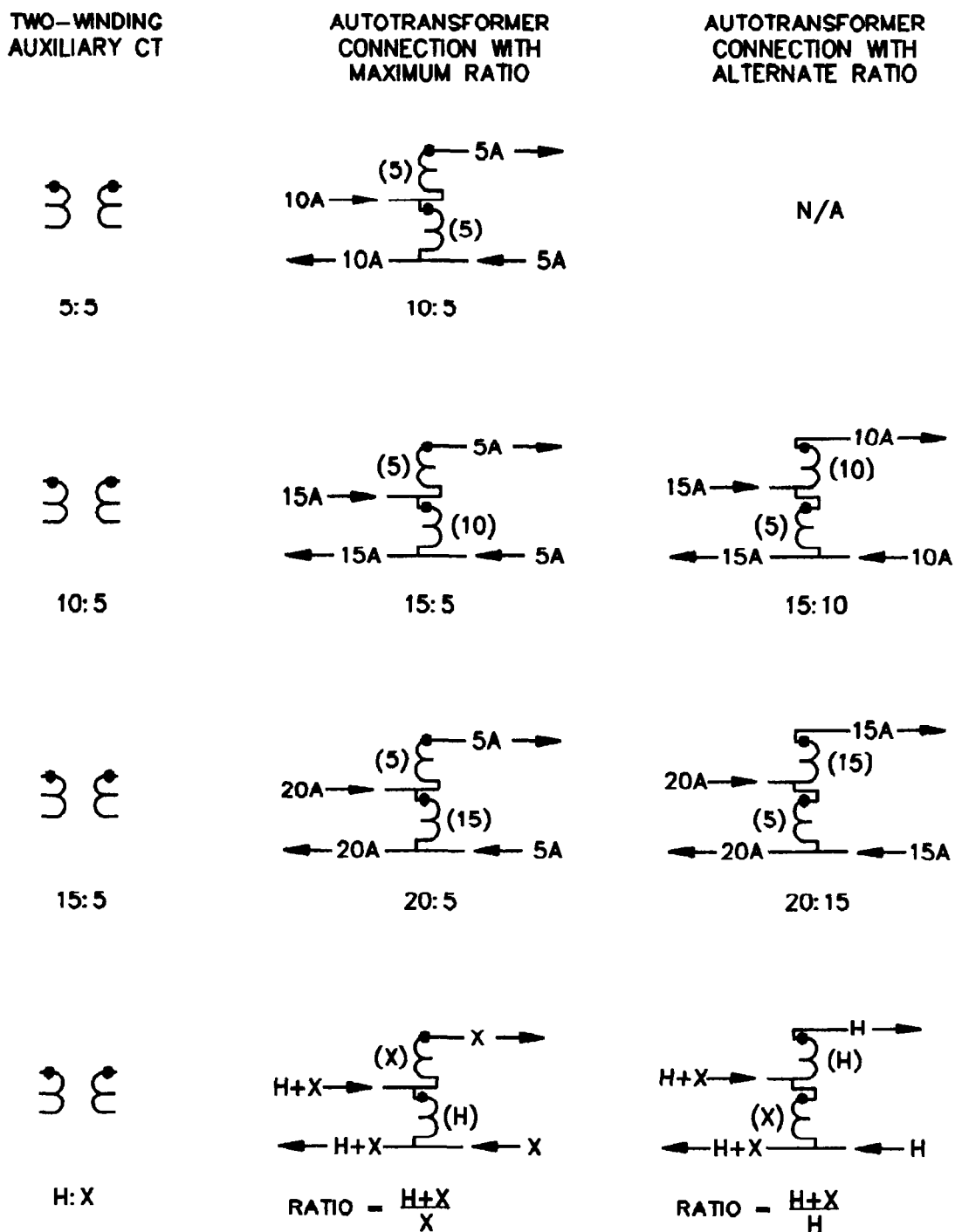
Figure 11—Two-winding auxiliary cts connected as autotransformers
