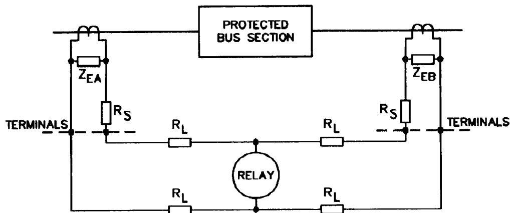
Figure 18—High-impedance bus protection
