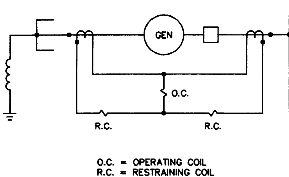
Figure 14—Generator differential application
