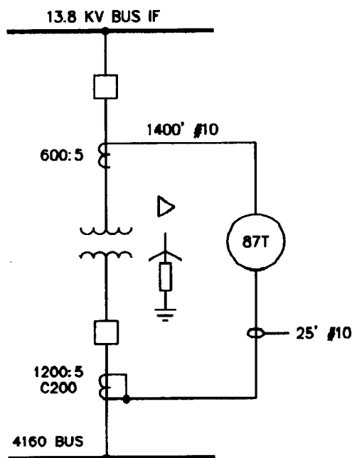
Figure 17—Transformer differential protection
