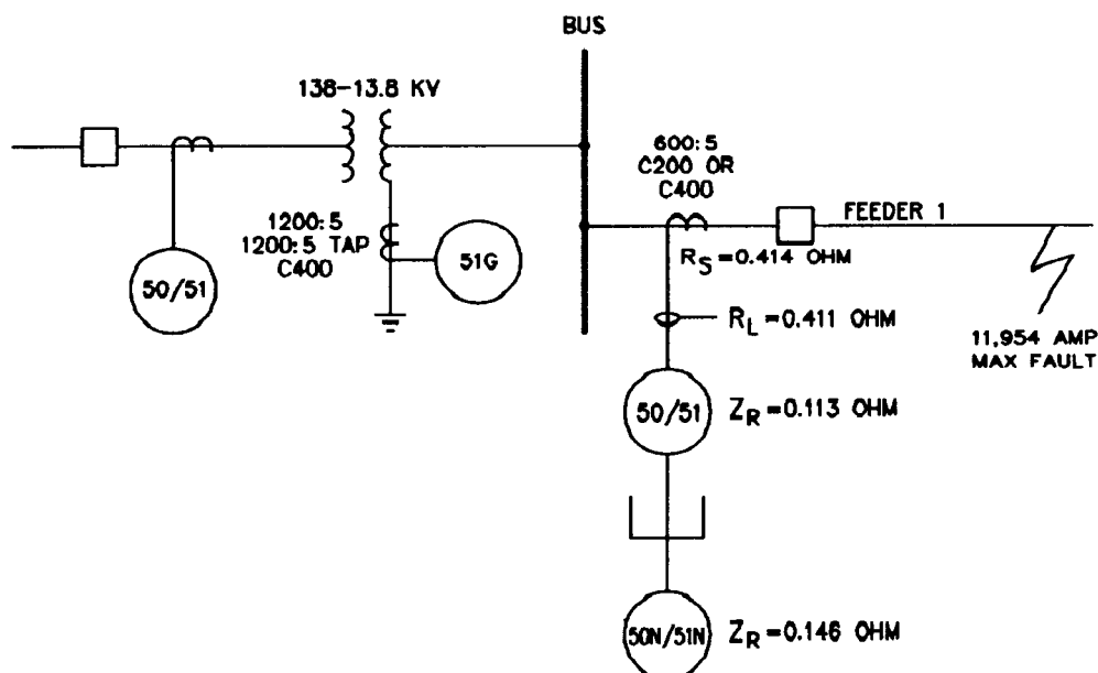
Figure 12—Nondirectional phase and ground overcurrent relays
