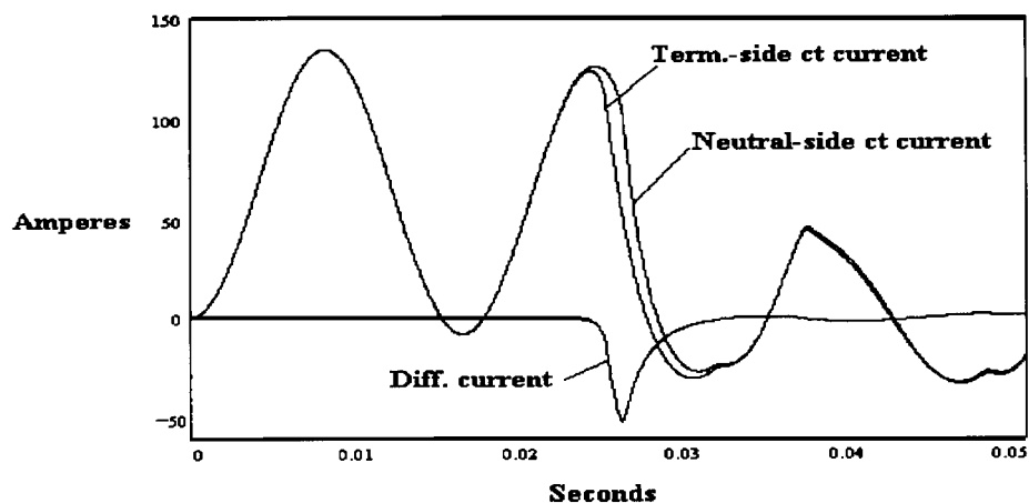
Figure 15—Secondary current in neutral and terminal side cts with differential current
