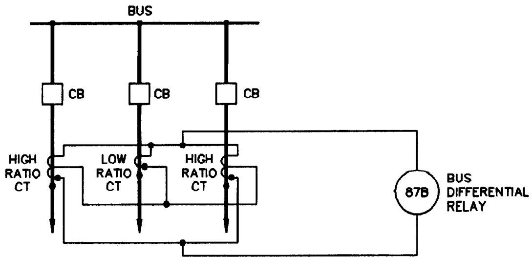
Figure 20—High-impedance bus differential
